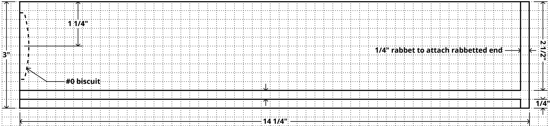
Toolbox side - lay out on 3 x 16 x 1/2" wood
